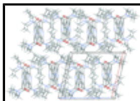
Fig. 2. Projection along the b axis with highlighted hydrogen bonds between the molecules in the bands in direction of c axis.
